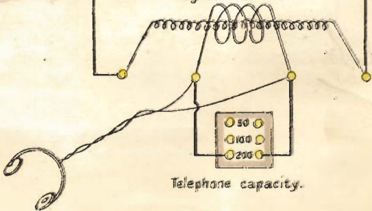
Magnetic Detector
