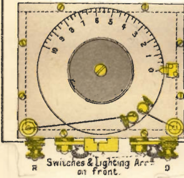
ACCEPTOR CONDENSER. HALF FULL SIZE.
